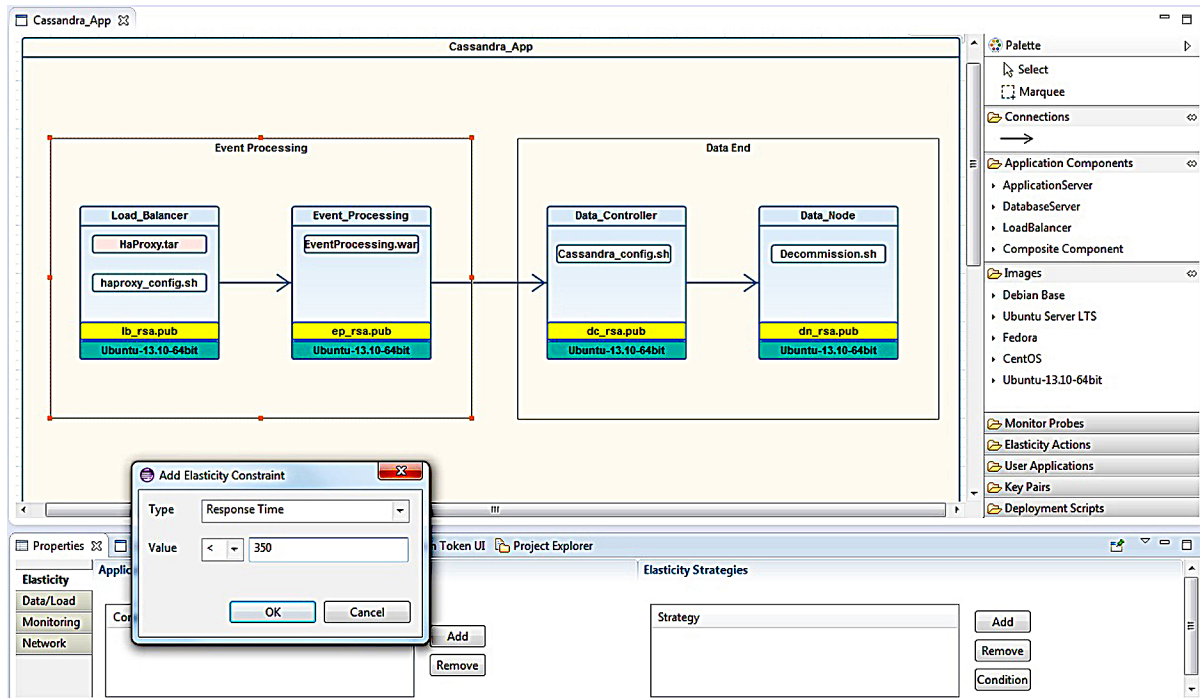
Figure 14. Application used for evaluation described in c-Eclipse
