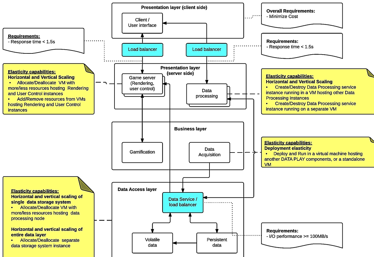
Figure 3. DataPlay application
