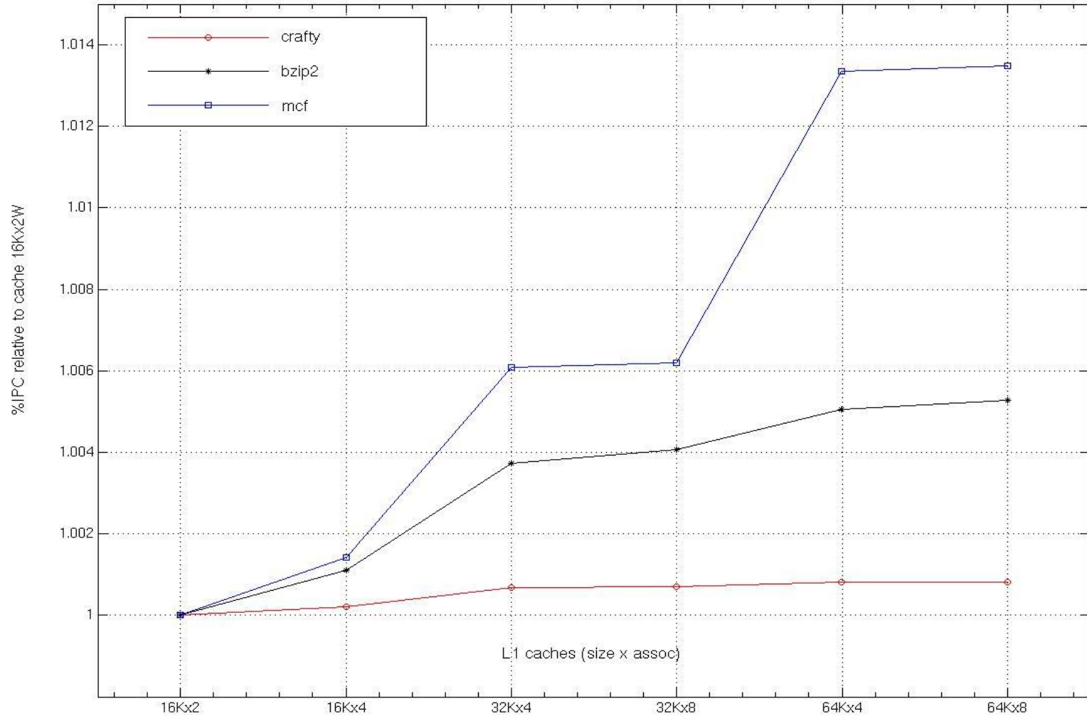
IPC for different L1 caches (block64)
